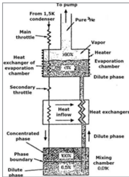
Figure 1: Typical diagram of the ^3\text{He}/^4\text{He} refrigerator
