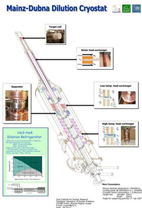
Figure 11: Main units and parameters of the polarized target cryostat in Mainz
