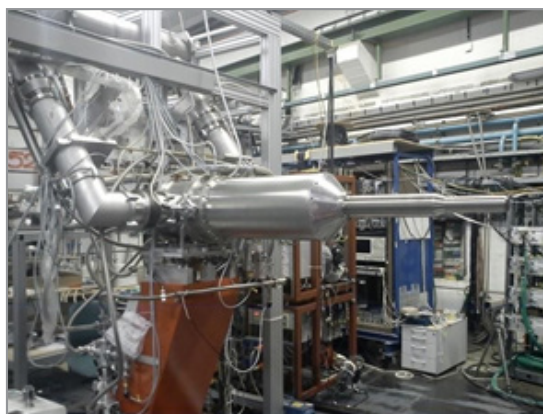
Figure 10: General view of the polarized target in the accelerator beam- line (MAMI C, Mainz)
