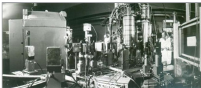
Figure 4: First frozen polarized target in the LNP synchrocyclotron beamline. A.S. Neganov, 1975
