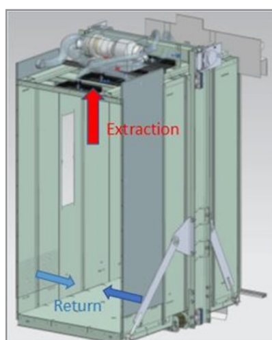
Figure 10: Schematic Representation of The Lift Cabin. The Ventilation Has an Air Exchange Rate of 27/H, The Mean Vertical Flow Velocity is 1.6 cm/s.
