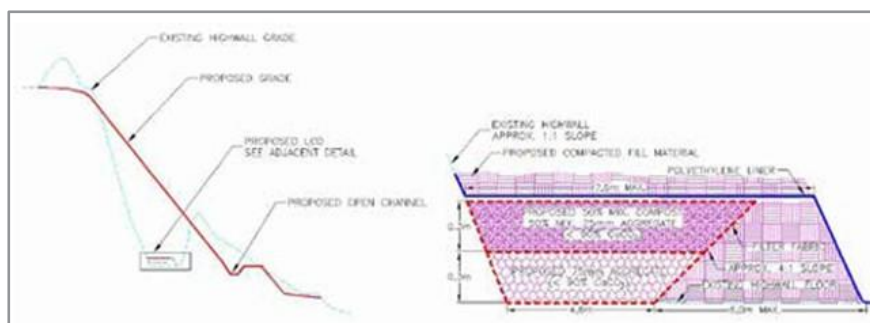
Figure 1: Lime Compost Drain (LCD), Typical Cross Section and Profile, Not to Scale (image: Olga Moya Aranzubia).
