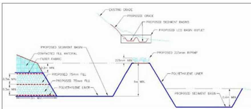
Figure 2: Lime Cost Drain Basin (LCD), Typical Cross Section and Profile, Not to Scale (image: Olga Moya Aranzubia).
