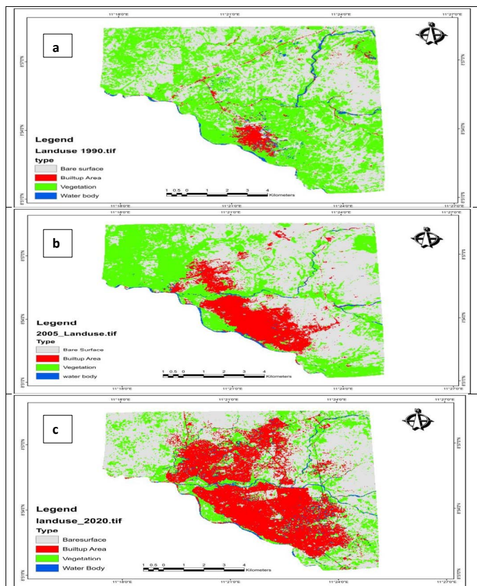
Figure 2: Land use and Land cover change of Jalingo in (a) 1990, (b) 2005 and (c) 2020
