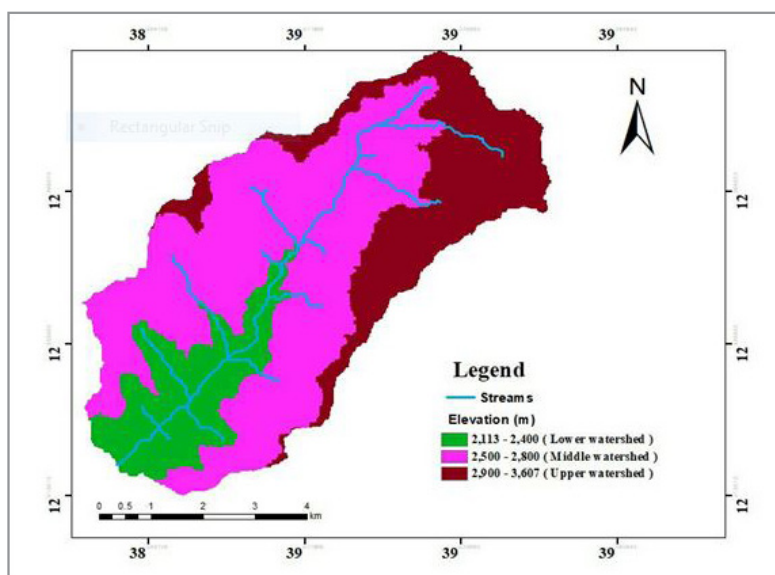
Figure 3: Elevation map of the study area
