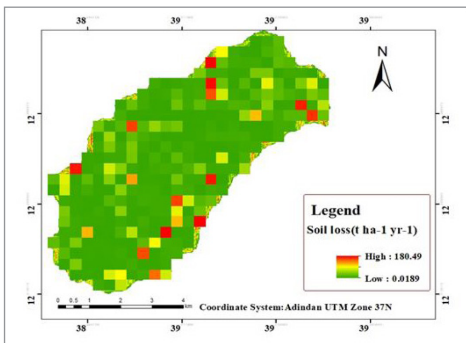
Figure 4: Soil Erosion map of the study area
