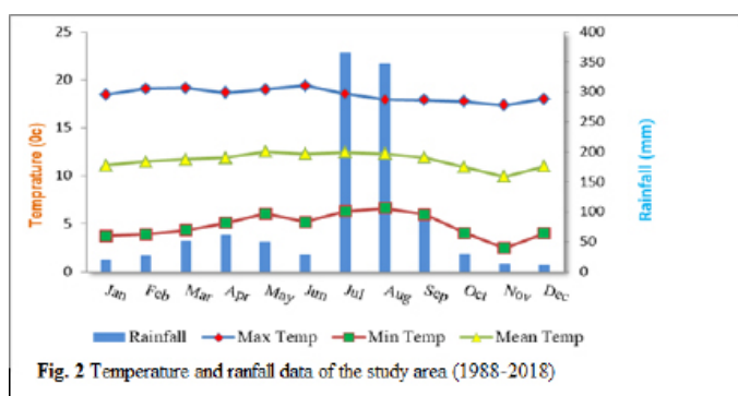
Figure 2: Temperature and rainfall data of the study area (1988-2018)
