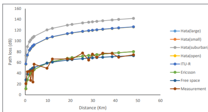
Figure 8: Generalised path loss model for route A
