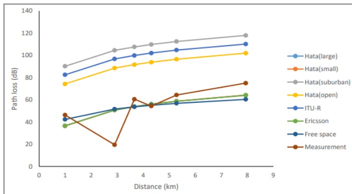
Figure 6: Modified path loss model for route B
