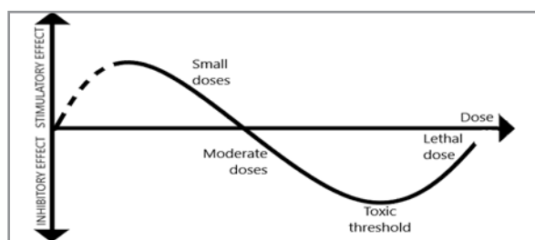
Figure 15: Arndt-Schultz Law
