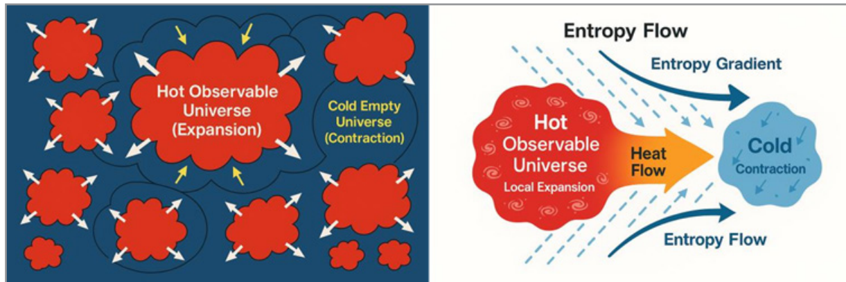
Figure 1: Illustrations by Mika G. Menken: (a) mosaic of hot, expanding regions versus cold, contracting voids; (b) heat- and entropy flow from a hot cell to a neighboring cold cell in the TGC framework.
