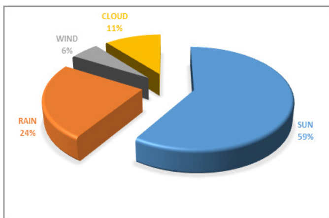
Figure 5: Atmospheric conditions
