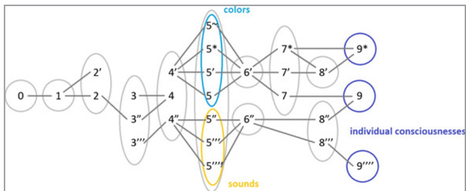
Figure 6: The intricacies of Self-Reference's levels
