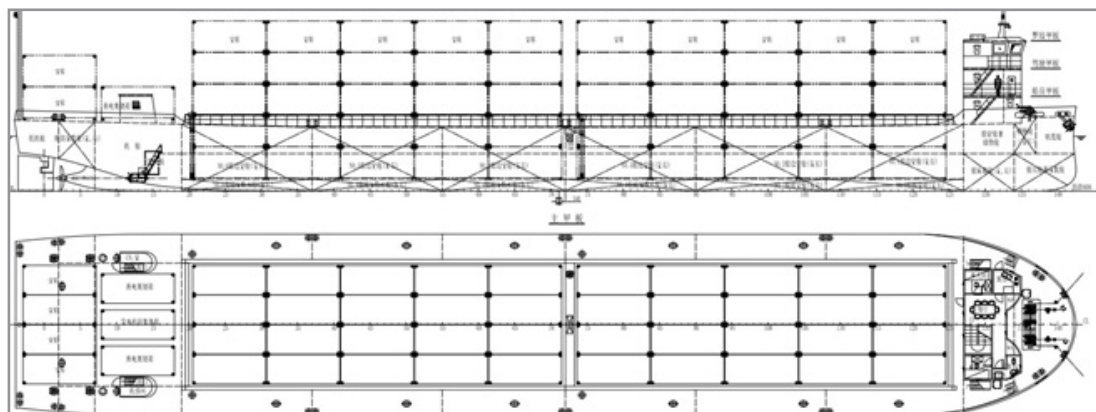
Figure 2: Schematic Diagram of the Overall Layout of the Demonstration Ship
