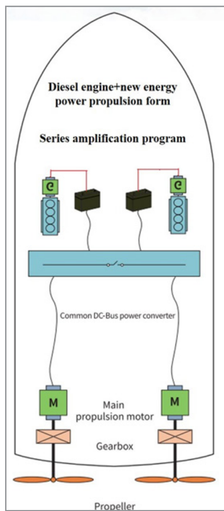
Figure 3: Series Extended Range Hybrid Mode
