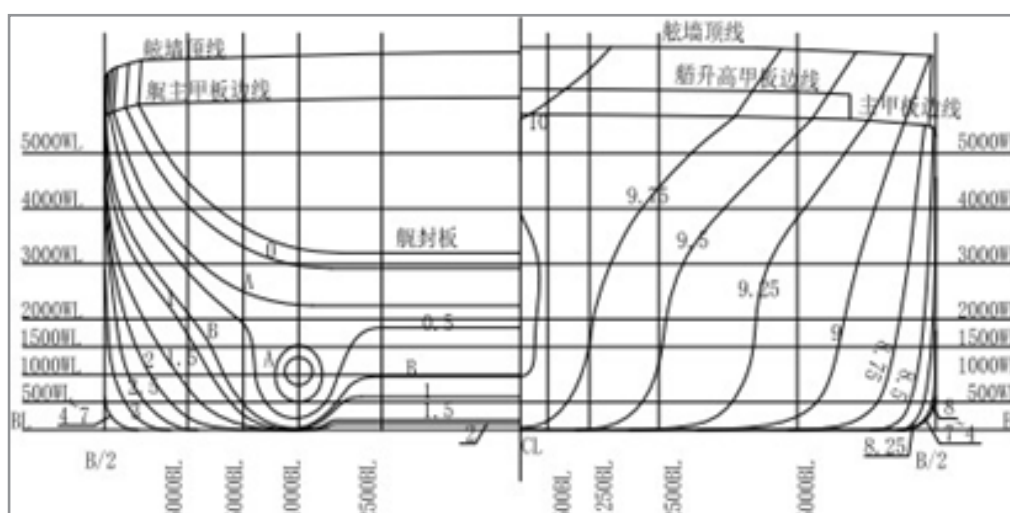
Figure 1: Schematic diagram of demonstration ship type line
