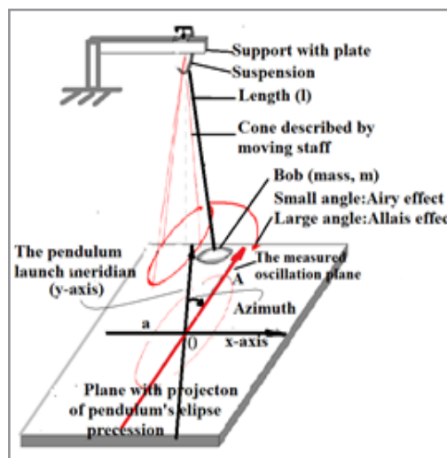
Figure 2: Constructive and dynamic elements of the paraconical pendulum in the Newtonian paradigm of experiment design
