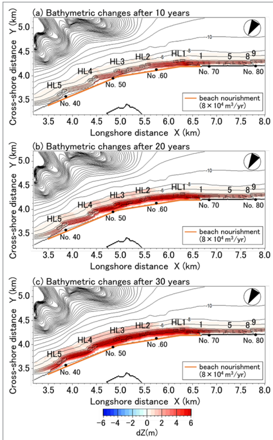
Figure 14: Topographic changes 10, 20 and 30 years from the present (Case 2).
