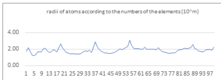
Figure 1: The radii of atoms in 10^{-9} m
