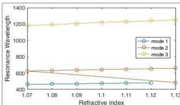
Fig 4: Resonance wavelength versus refractive index changes.
