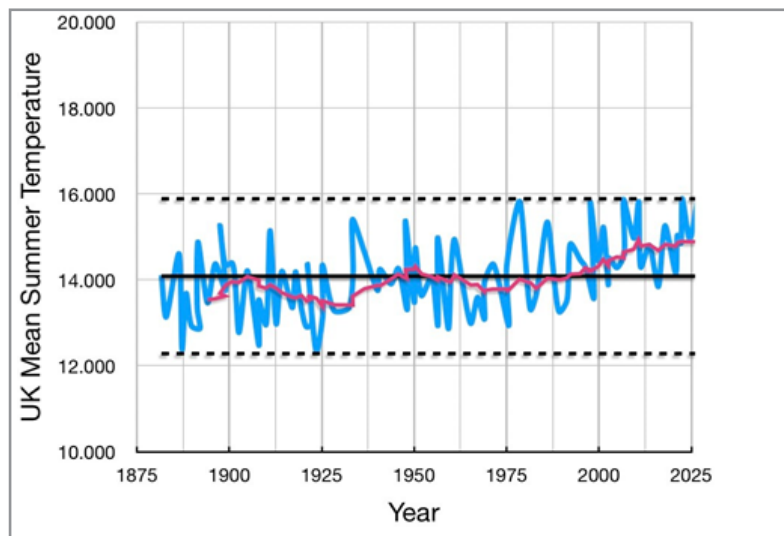
Figure 2: Mean UK Summer Temperature with mean and standard deviations
