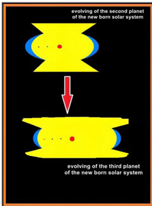
Figure 5: The Formation of the Second and Third Planet of the New Born Solar System and its Expanding.
