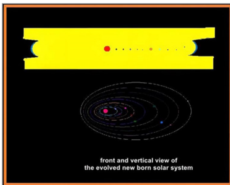
Figure 6: The Finishing of the New Born Solar System.
