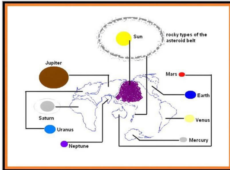
Figure 7: The Corresponding Relationship between the Main Celestial Bodies of the Solar System and the Ancient Plates Group of the Earth.
