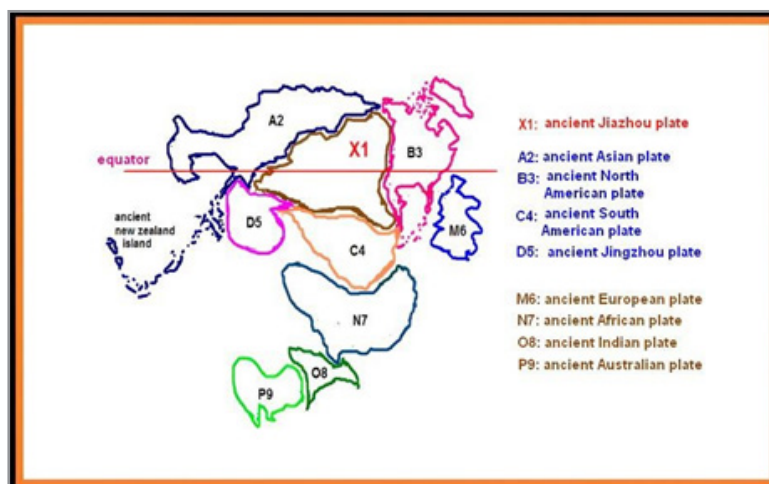
Figure 9. the jigsaw recovery of the supercontinent of the planet Earth.
