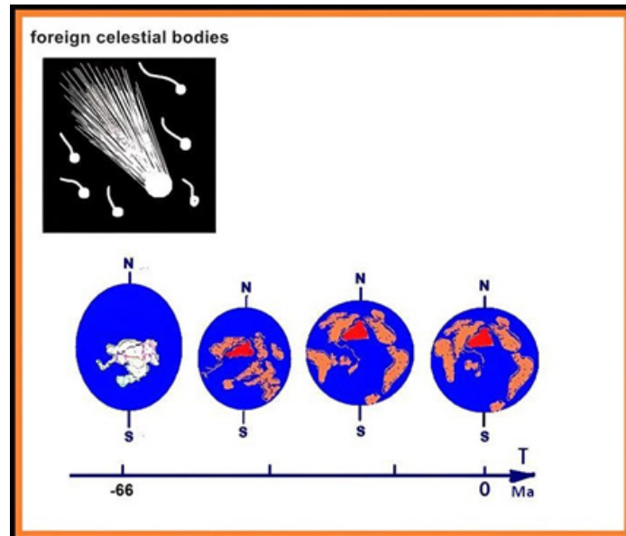
Figure 11: The Evolving Process of The Unique Supercontinent from 66 Million Years before.
