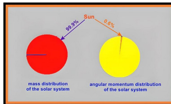
Figure 2: The Contrast Extremity of the Mass and Angular Momentum of The Sun of the Solar System.
