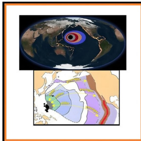
Figure 8: The Hint Black Hole (Hbh) Hidden on the Ocean Floor of the Northwestern Pacific Ocean.
