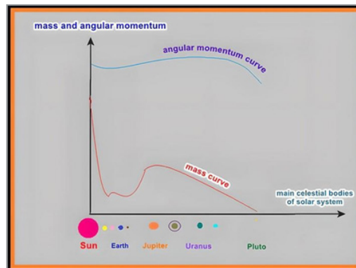
Figure 1: The Mass and Angular Momentum Distribution of the Celestial Bodies of the Solar System.
