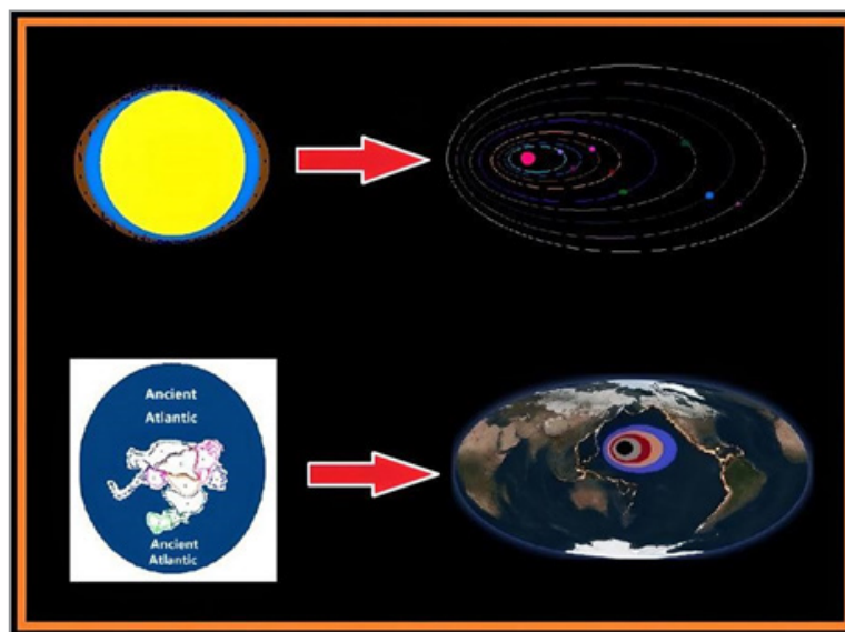
Figure 12: The Similar Evolving Pattern Between the Birth of the Solar System and the Ancient Plates Group of the Earth.
