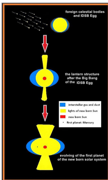
Figure 4: The Big Bang of the Idsb Egg and the Evolving of the First Planet of the New Born Solar System.
