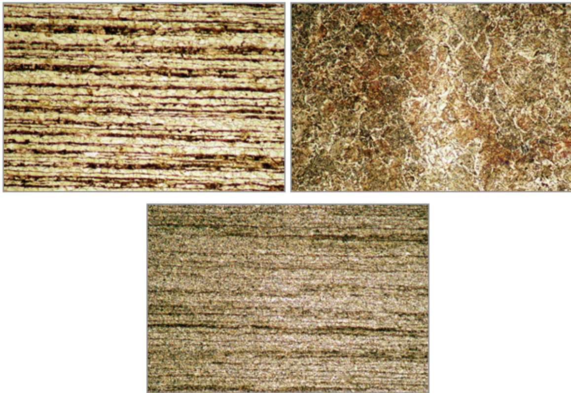
Figure 5: A Base Metal, Part 1, B Weld Metal And Haz, C Base Metal Part 2 (a-c) x50 Microstructure of the welded joint part 1
