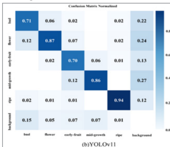
Figure 9: Confusion matrix for YOLOv11.
