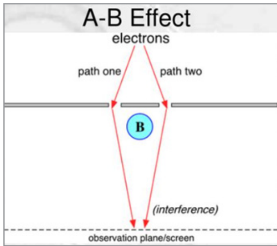
Figure-1(b): Illustration of Interference Experiment for Aharonov-Bohm Effect with Solenoid Inducing Magnetic Field
