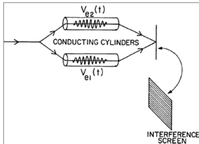
Figure 1(d): Electric AB effect. V1e=V2e=0 except when the wave packet is shielded from the Electric the Electric Field
