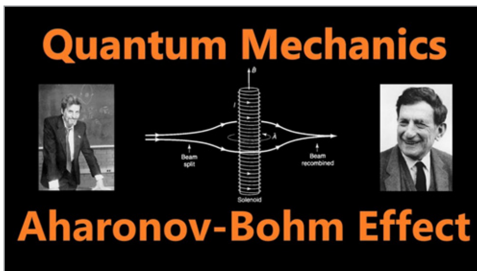
Figure-1(a): Aharonov-Bohm Effect
