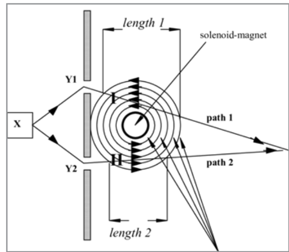
Figure-1(c): Two-Slit Diffraction Experiment of the Aharonov-Bohm Effect
