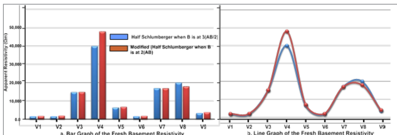
Figure 9: The bar Chart Graph of the Fresh Basement Resistivity of the Study Area
