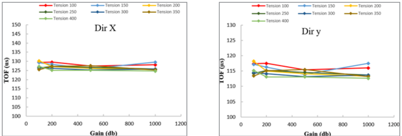
Figure 3: TOF as a Function of Gain and Voltage
