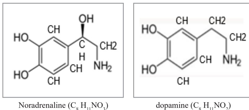
Figure 4: Structure and element-bond in noradrenaline and dopamine
