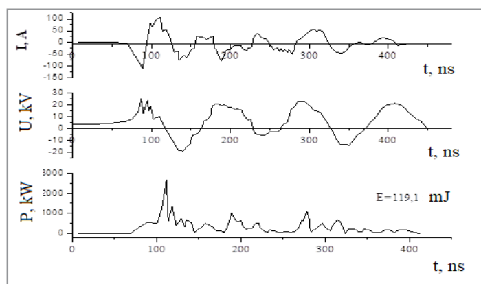
Fig 1: Oscillograms of current pulses, voltages, pulse power and energy contribution to an overvoltage nanosecond discharge for one pulse ( p(\text{Ar}) = 101 kPa, f = 1000 Hz, d = 2 mm).
