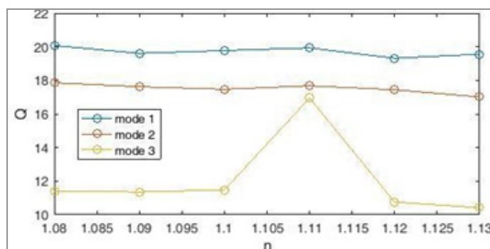
Fig 7: Diagram of quality coefficient Q of plasmonic sensor.
