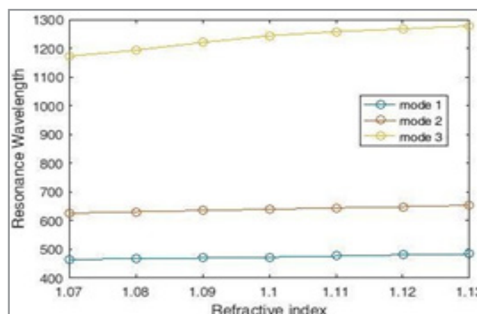
Fig 11: Resonance wavelength versus refractive index changes.
